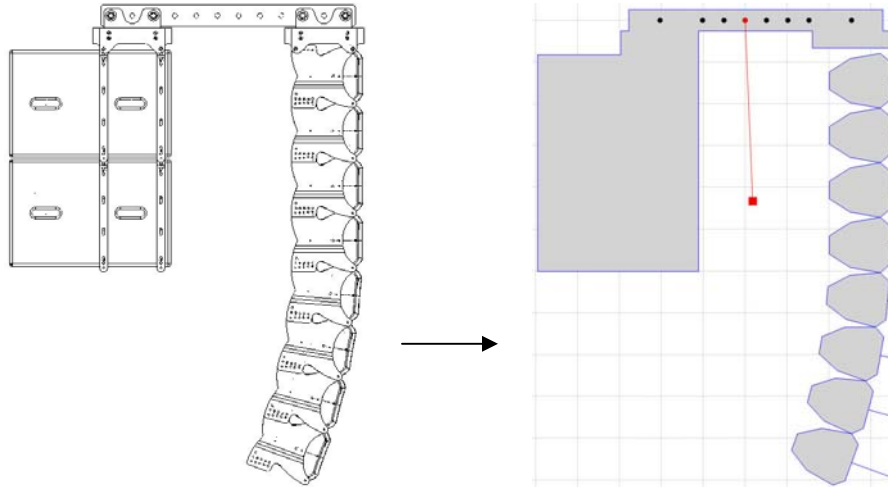
Figure 1 – Array shown with 2 subs behind primary array
