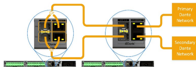
Figure 7 - "Redundant" mode with daisy chaining
