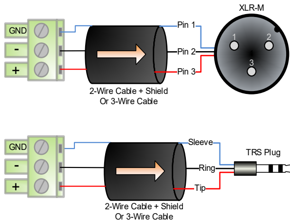
Figure 11 - AXP20 to Balanced Input Wiring Guide
