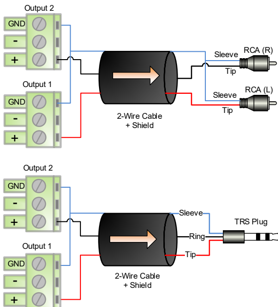
Figure 12 - AXP20 to Unbalanced Input Wiring Guide
