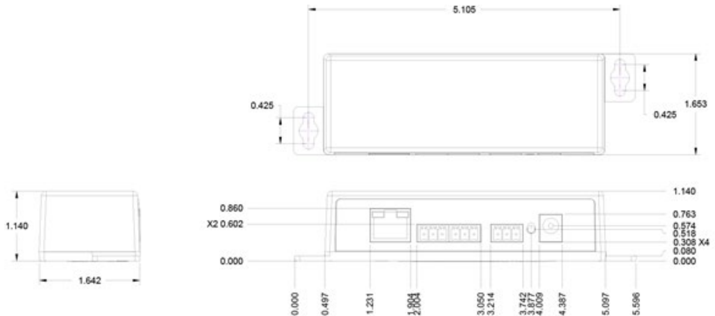
Figure 10 - AXP2O Dimensional Drawings
