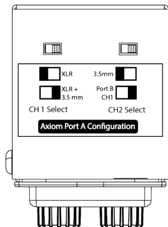
Figure 6 - Switch Label/Config Options
